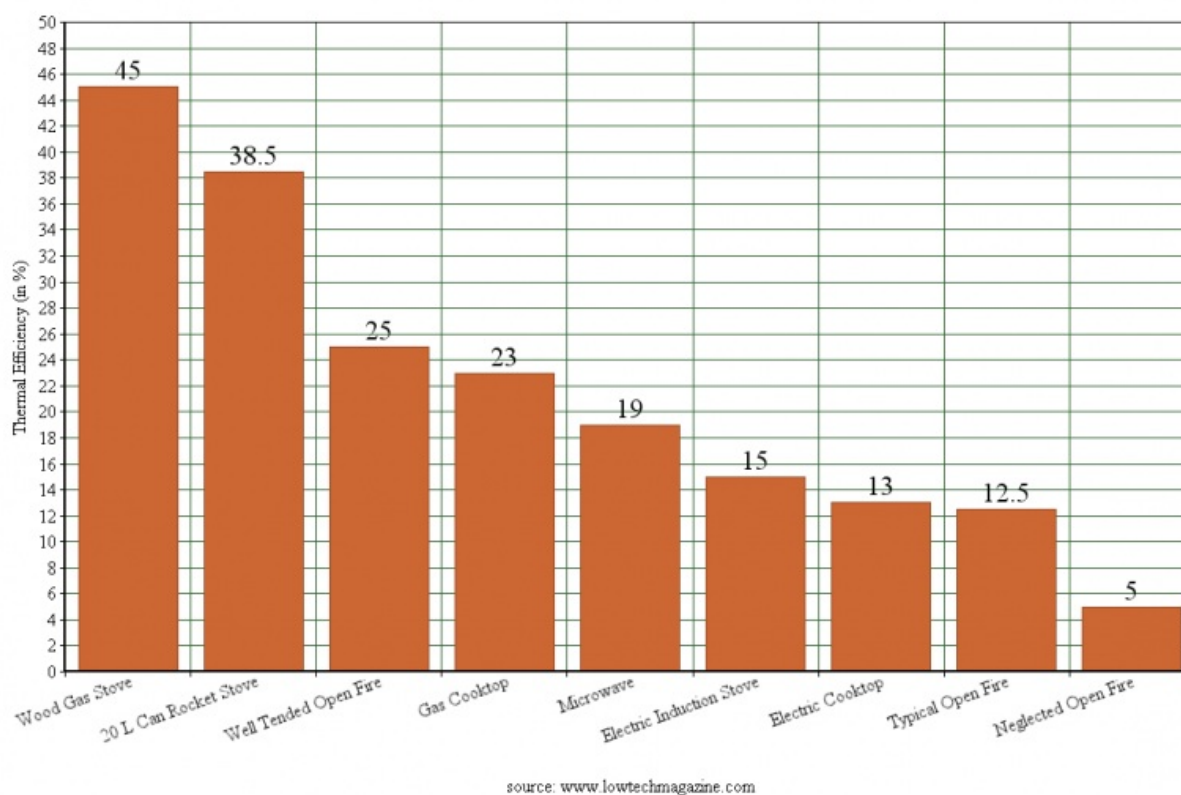
Thermal Efficiencies of Cooking Appliances in Poor & Rich Countries
